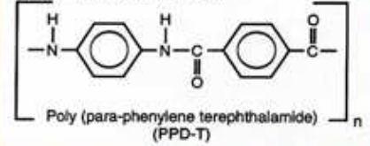
Kevlar® Para-Aramid Fiber
